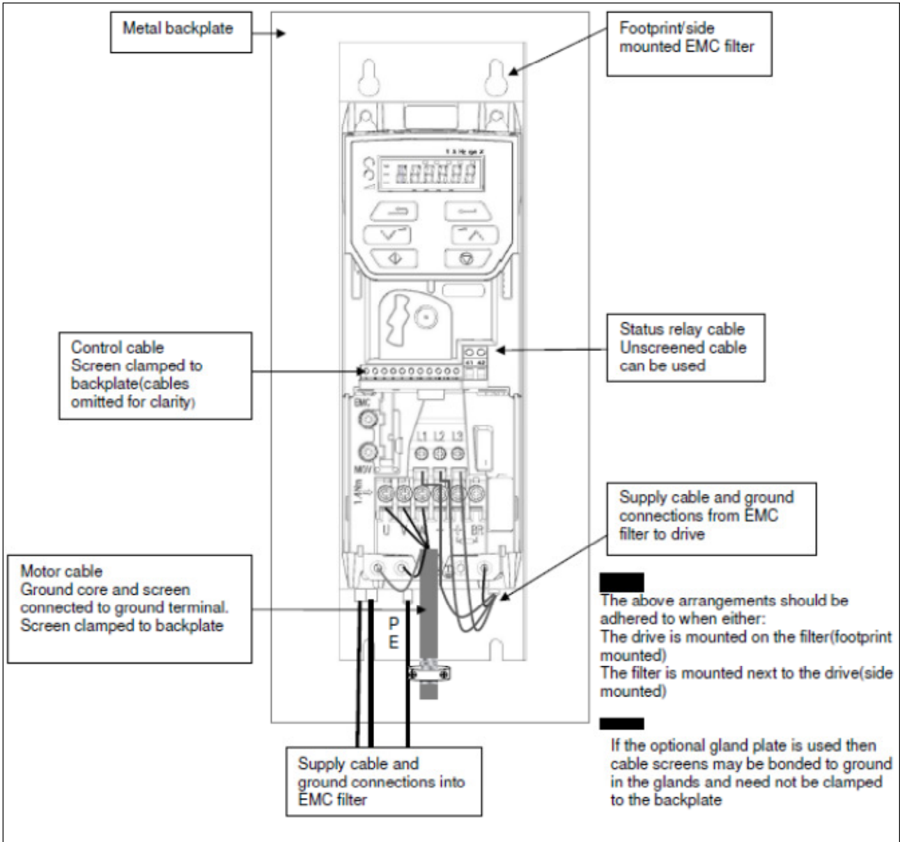
Figure 4 Wiring guidelines
